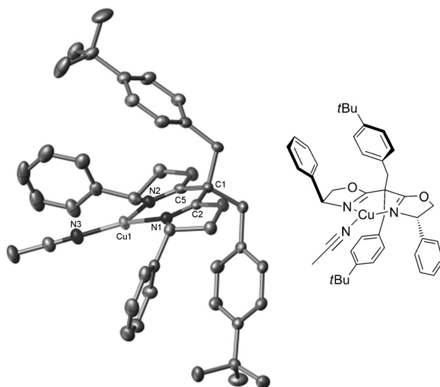
Figure 1. X-ray structure of [Cu( L4 )(CH 3 CN)] + (unless labeled, hydrogen atoms and PF 6 − are omitted for clarity).
